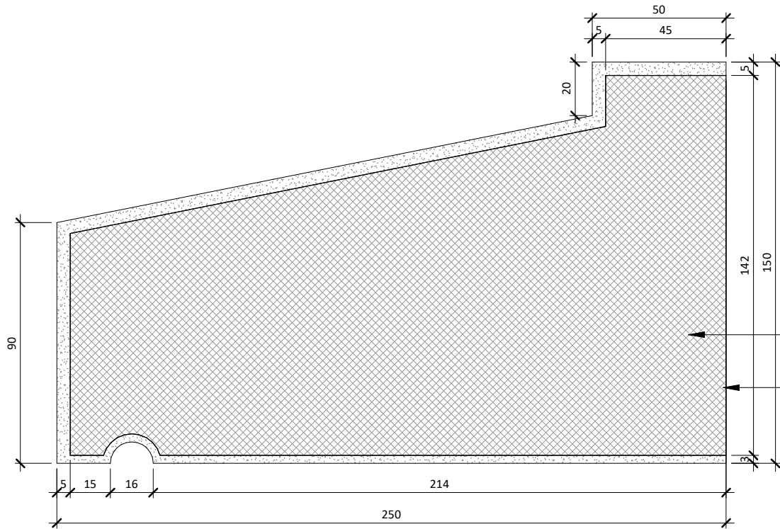
1 250mm Sill S-03 1 : 2
